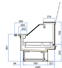
Dream ST P90 / H125 TCB L93-125
